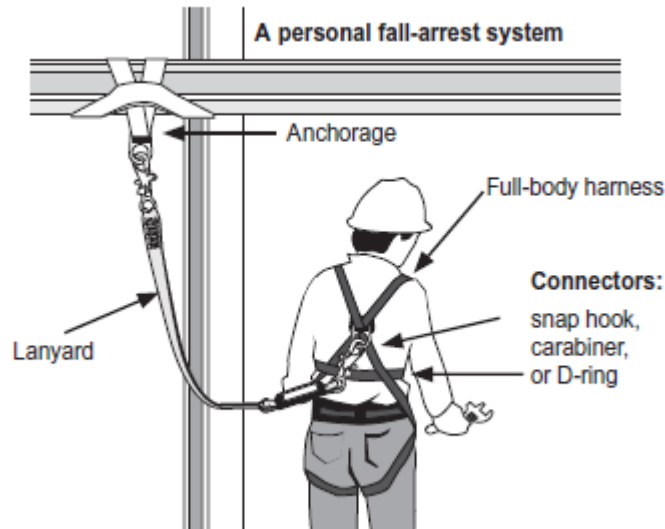
Example of the type of personal fall arrest system employed at RWU
