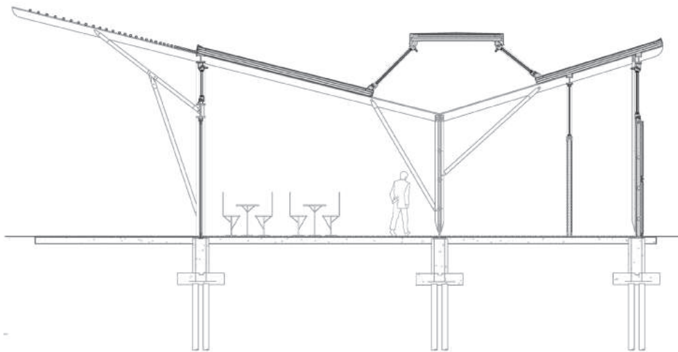
Providence River Side Pavilion Structural Model and Section
