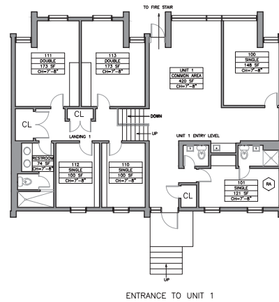
1 UNIT 1 – ENTRY LEVEL AND 1ST LANDING 1,606± sq. ft.
